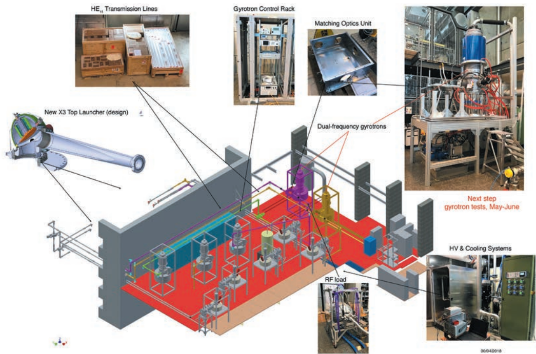
TCV EC-system with dual-frequency gyrotrons included. Depending on the frequency generated (126 or 84GHz), the mm-wave radiation is directed via the Matching Optics Unit towards the corresponding existing transmission lines for top-launch (X3@126GHz) or low-field-side launch (X2@82.7/84GHz or X3@118GHz). The insets showing the first dual-frequency gyrotron with different gyrotron auxiliaries: control and protection units, High-Voltage and cooling systems, Matching Optics Unit, high-power calorimeter (rf load), the transmission lines and the design of the X3 top launcher.
